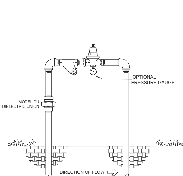
HORIZONTAL INSTALLATION
