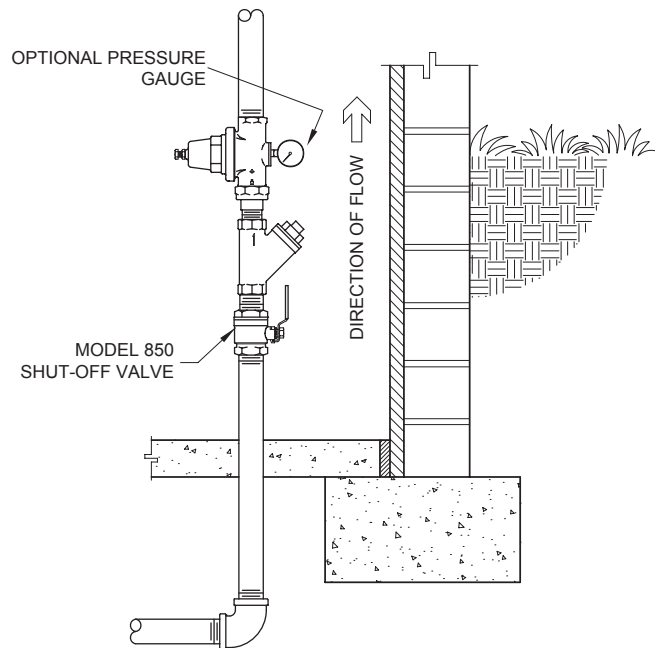
VERTICAL INSTALLATION
