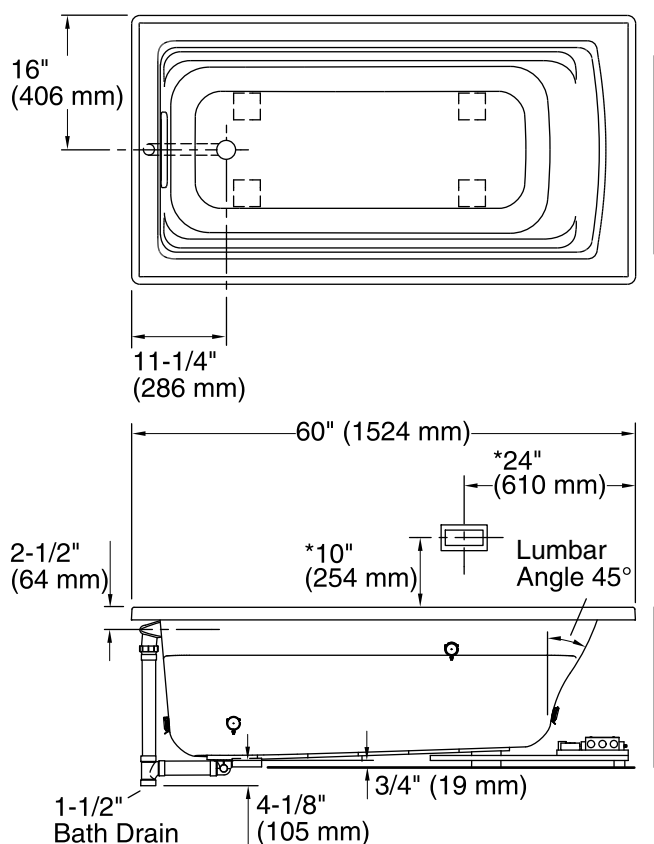
Access Panel 30" (762 mm) W x 15" (381 mm) H Min
