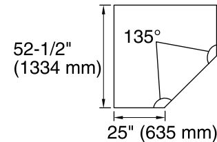
Cut-Out Detail
