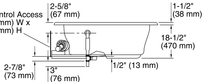
Cut-Out Detail
