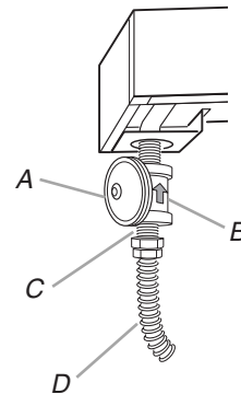
A. Gas pressure regulator B. Regulator - Must be installed with arrow pointing up to cooktop bottom C. Adapter - Must have \frac{1}{2} " male pipe thread D. CSA approved flexible stainless steel gas supply line
