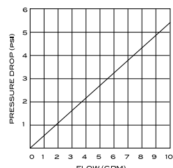
Depth Cartridge (5 micron)
