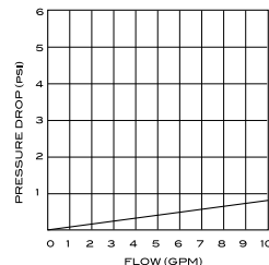
Pleated® Cartridge (5 micron)
