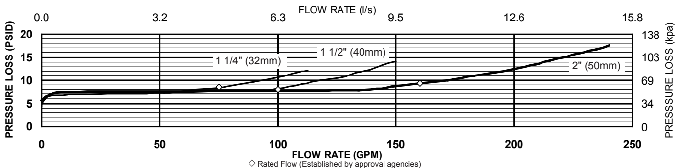
MODEL 950XLTBF(SS) 1-1/4", 1-1/2" & 2" (STANDARD AND METRIC) HORIZONTAL AND VERTICAL INSTALLATION
