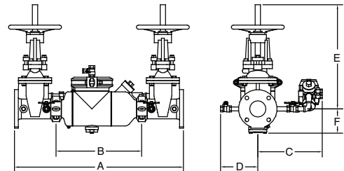
MODEL 350ASTDA with OS&Y option
