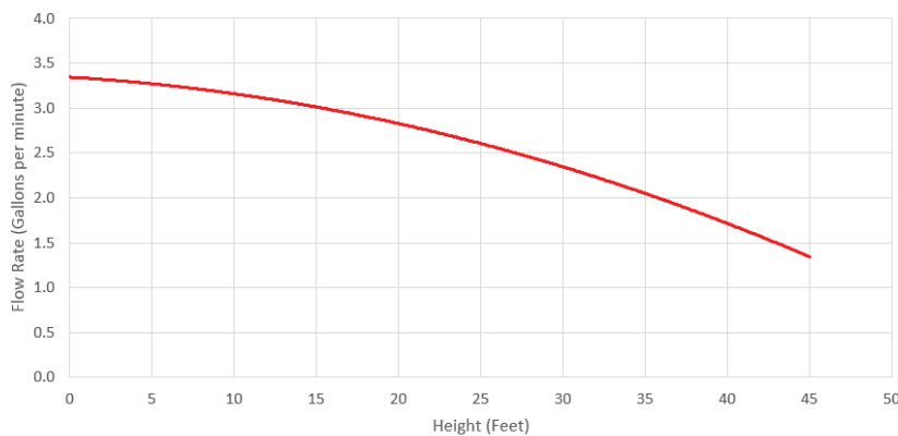
BP-46 Performance Curve
