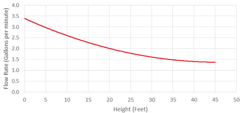
BP-46-230 230V Performance Curve
