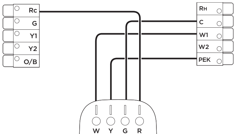
Power Extender Kit (at your HVAC system)
