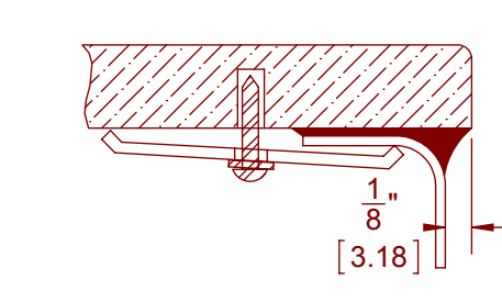
1/8" OVERHANG [3.2 SOBRESALIENTE]
