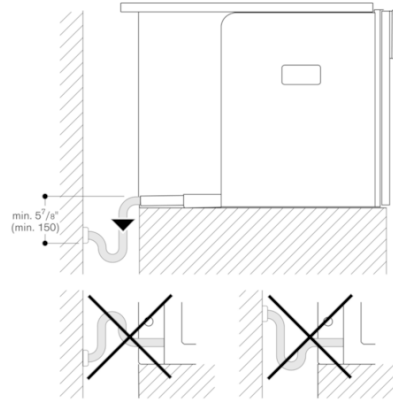
Drainage connection
