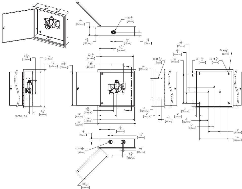
STW-SC3 RECESSED MOUNT ROUGH-IN DIAGRAM
