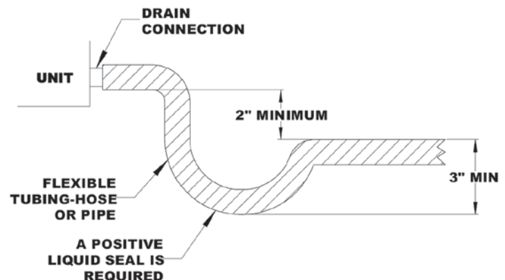
Fig 4-1. Typical drain line trap set up
