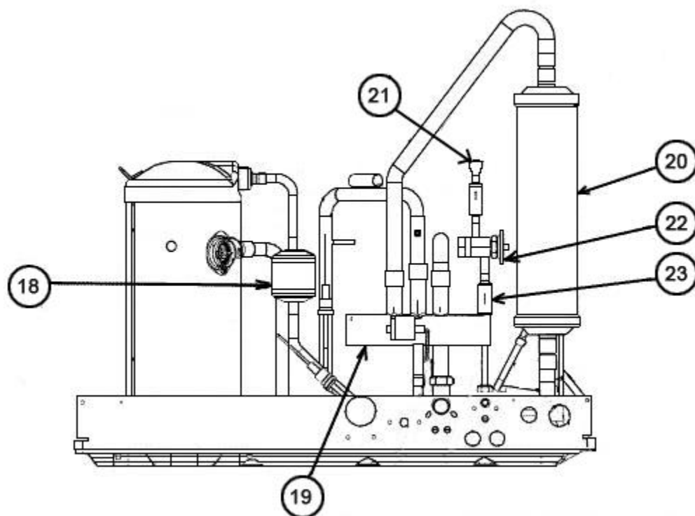
Compressor and Refrigeration Assembly
