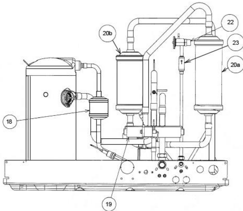
Compressor and Refrigeration Assembly (JEC 036 after 2909)
