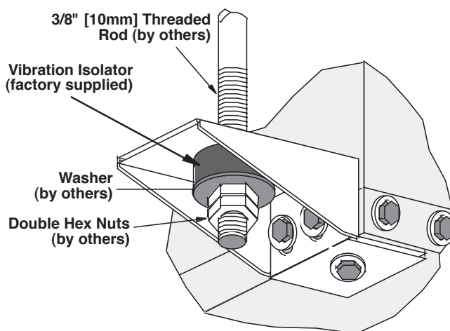
Figure 1: Hanger Bracket
