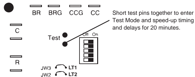
Figure 23: Test Mode Pins
