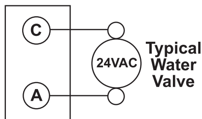
Figure 19: Accessory Wiring
