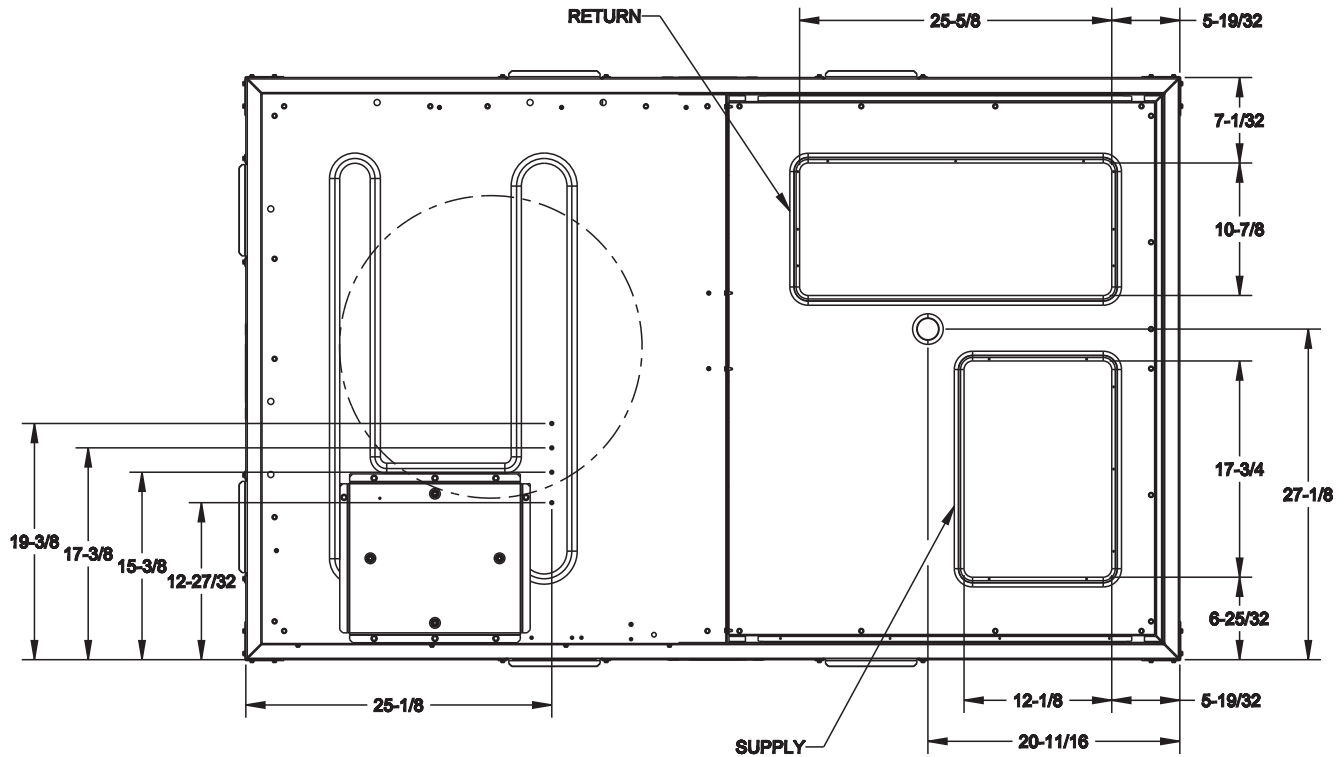
Figure 3. Cooling with optional electrical heat and gas/electric units — plan view — 3–5 tons
