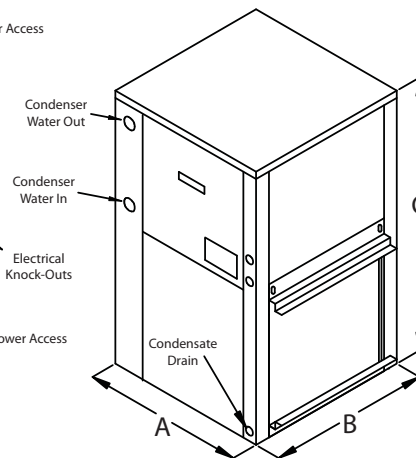
Right Hand Return (FRB)
