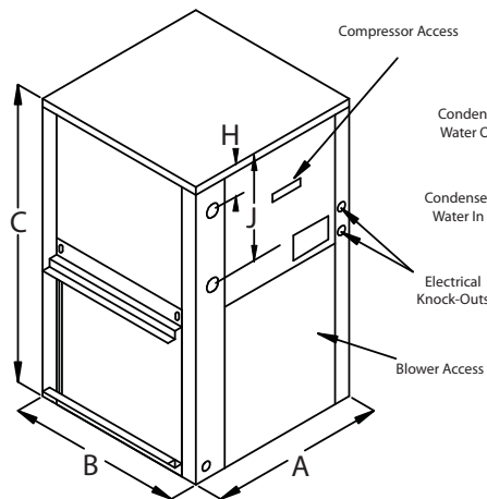
Left Hand Return (FLB)
