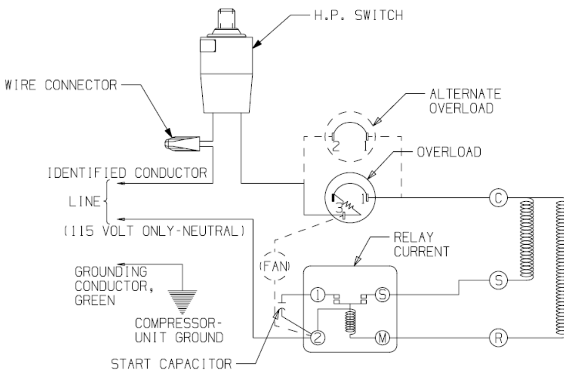
115 OR 230 V SCHEMATIC WIRING DIAGRAM - CSIR
