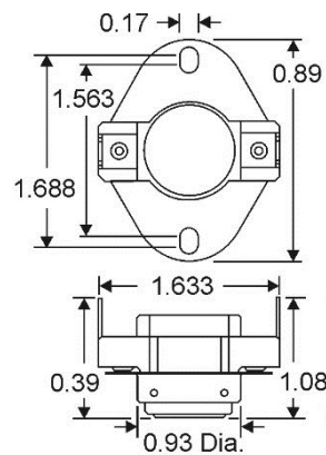
Air Stream Mounting
