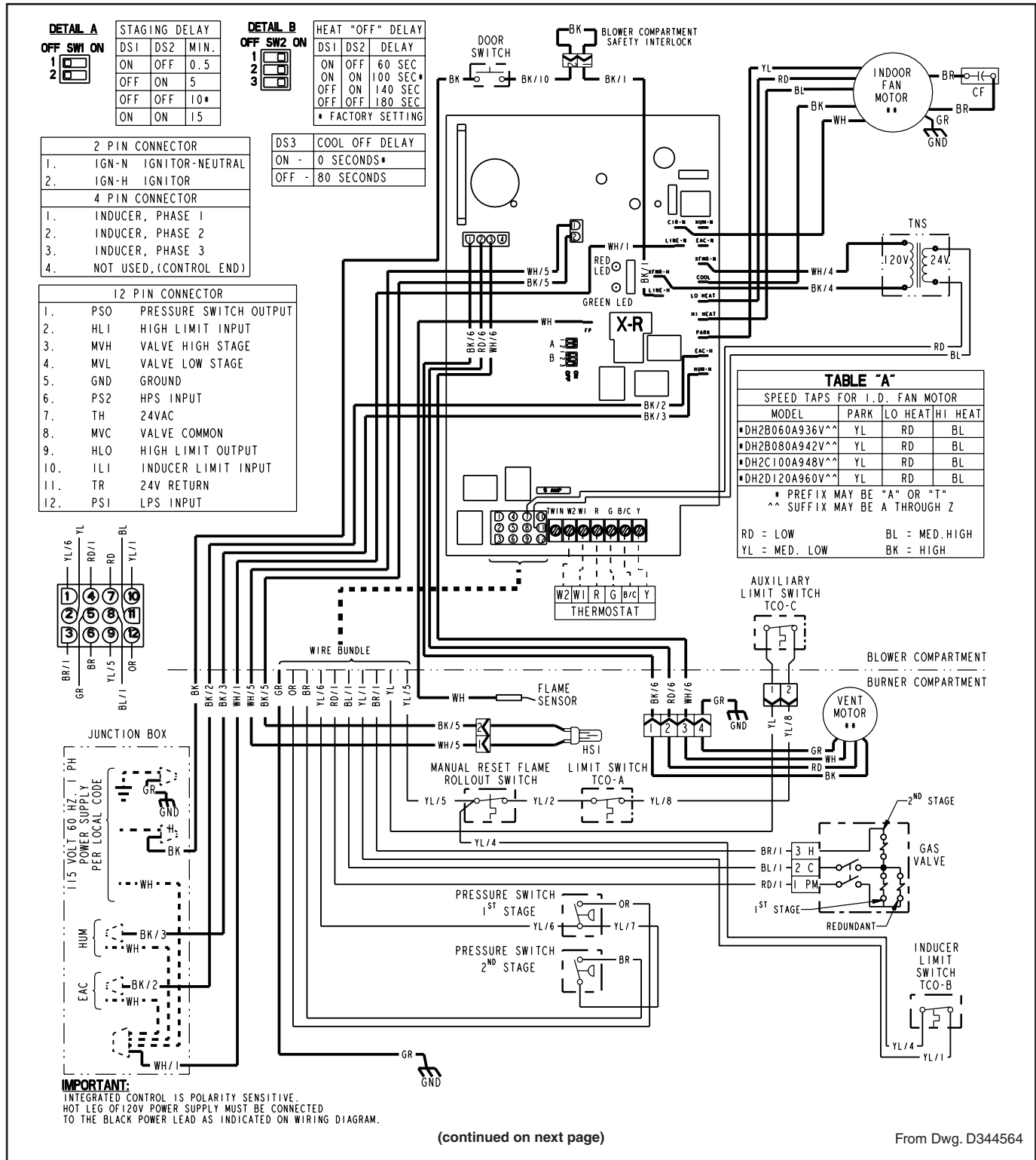
*DH2 Wiring Diagram
