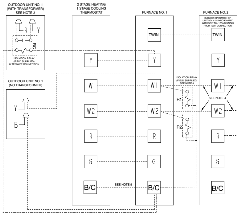
TWINNING CONNECTION DIAGRAM FOR TWINNING UX/DX-R FURNACES 2 STAGE HEAT / 1 STAGE COOLING THERMOSTAT
