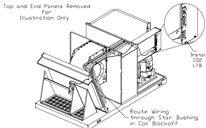
Figure 1. Panel removal
