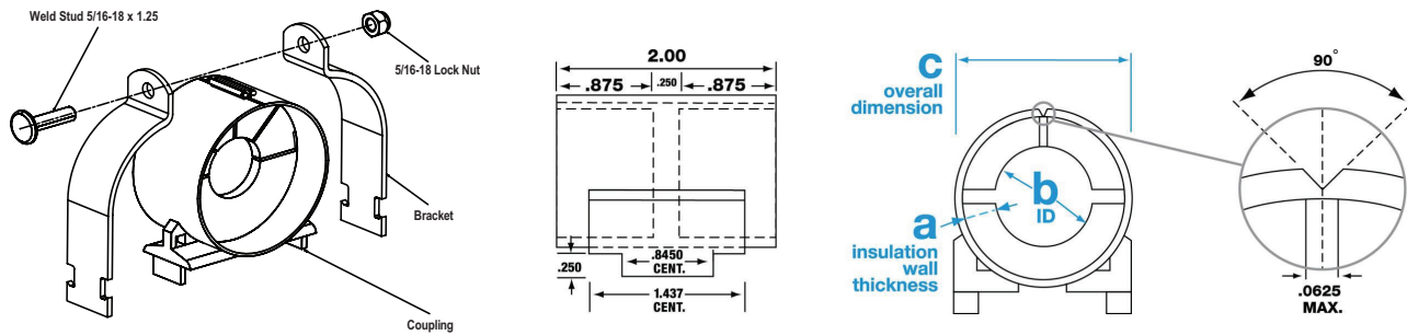
FIGURE 7899 - Insulation Couplings
