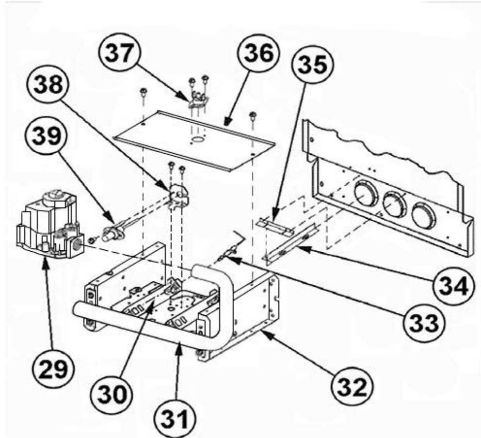
Burner Assembly
