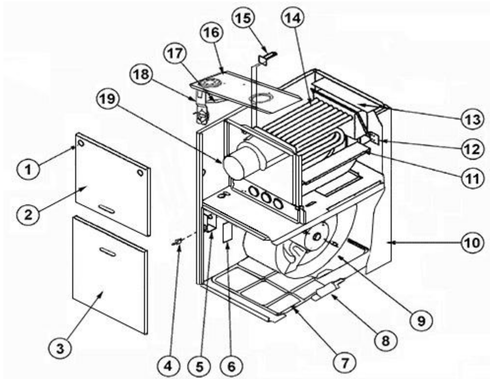
Exploded View
