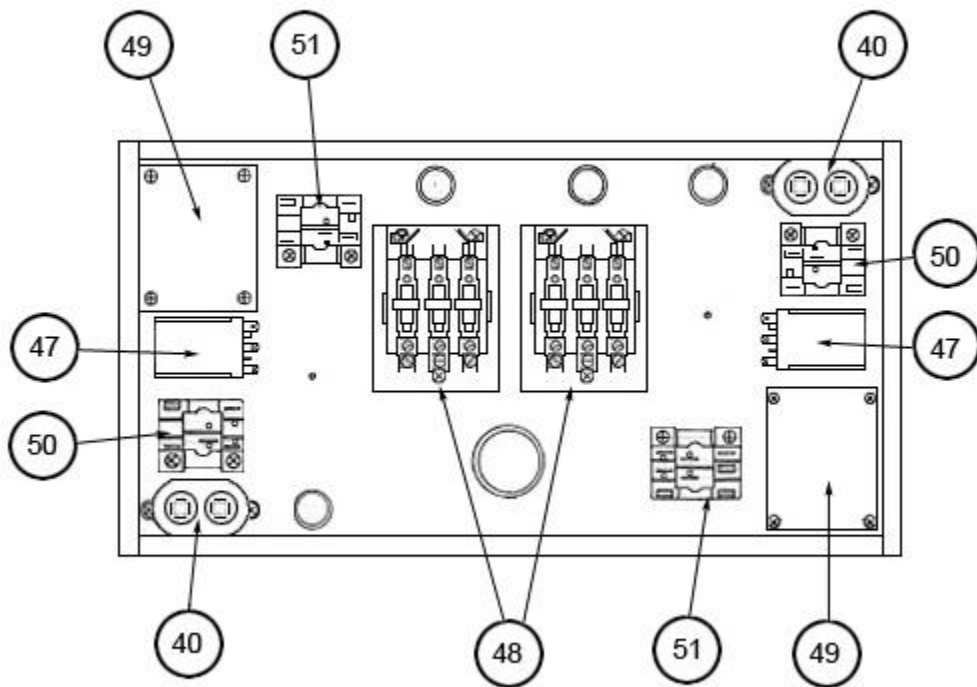
Control Box Condensor 075-100
