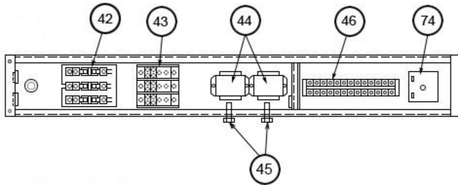
Main Control Box
