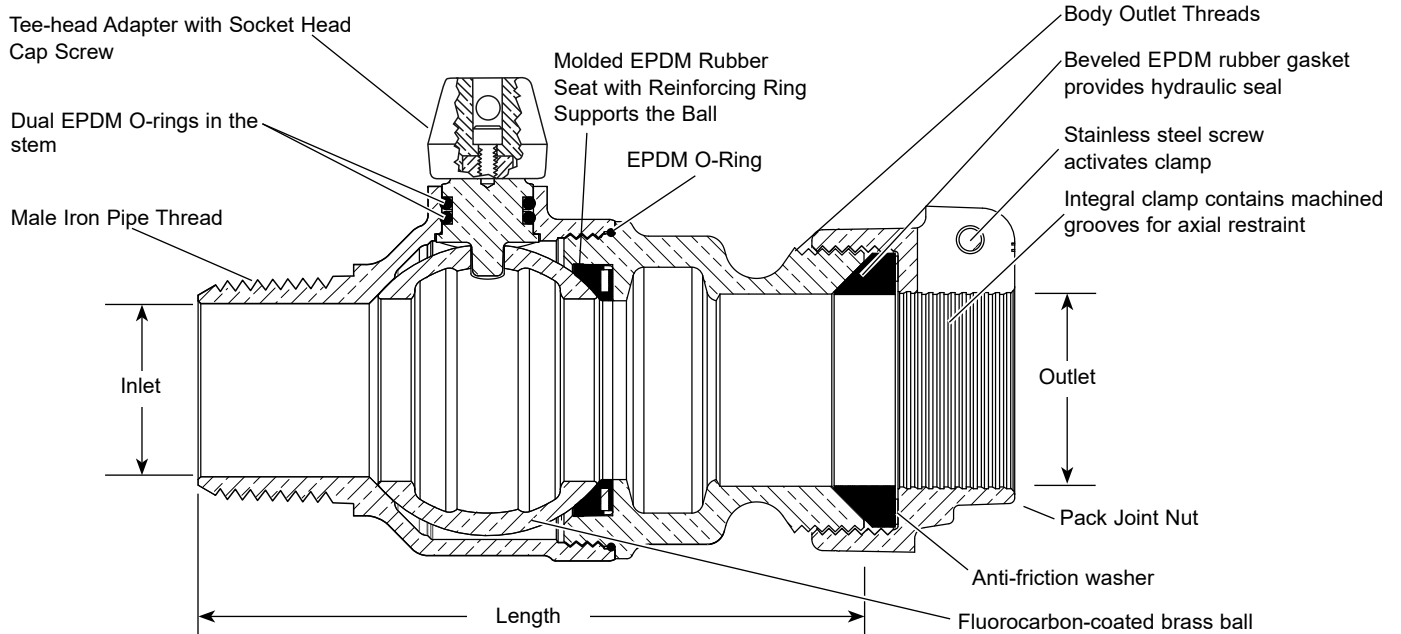
Image shown above is an FB1100-7-TA-NL.
