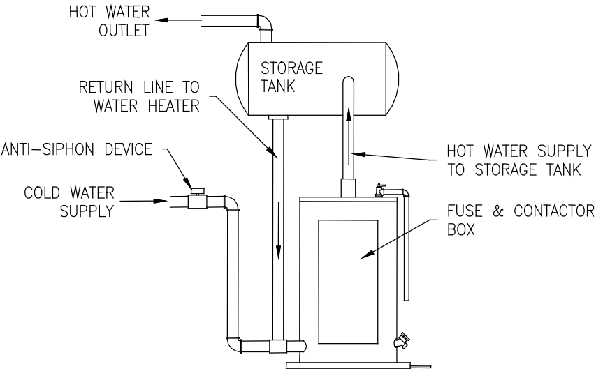
Figure 3A (Single Installation With Storage Tank Gravity Circulation) 50A, 80A, 120A
