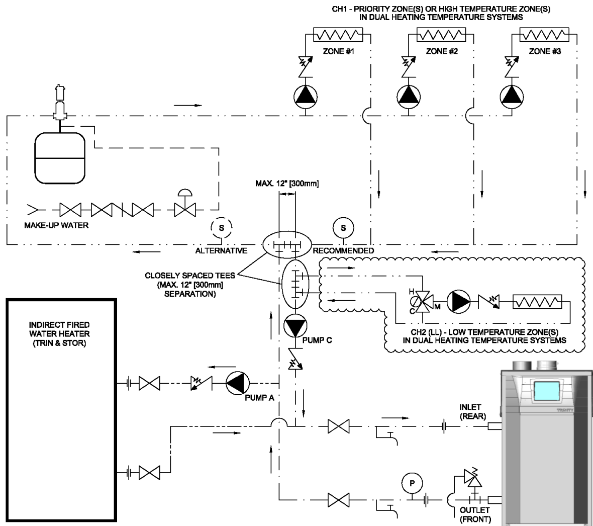
Stand Alone Boiler Plumbing Primary/Secondary Loop (Multiple System Circulator Configuration)
