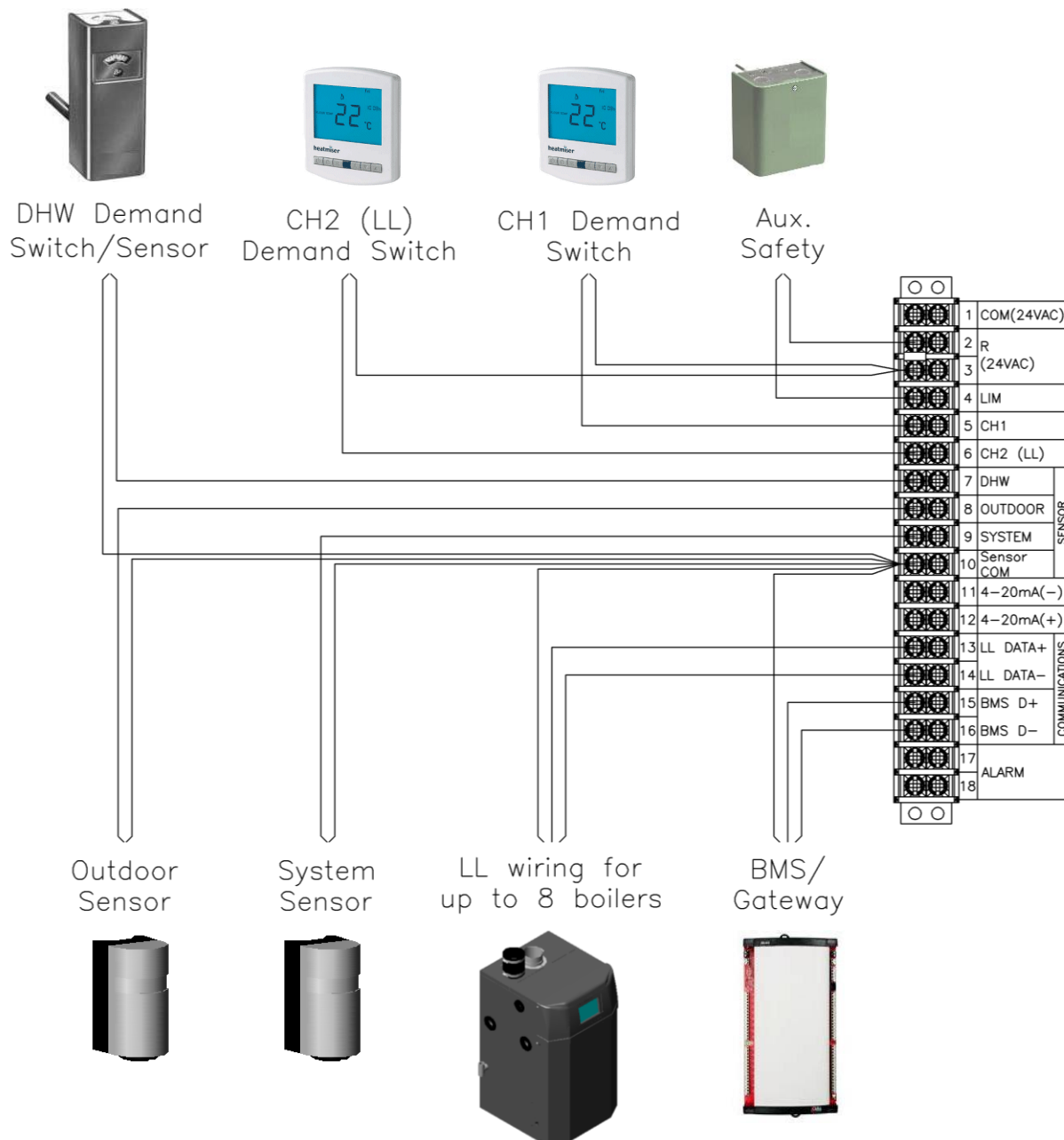
Figure 3-2 All Models (Lx150-400 shown)
