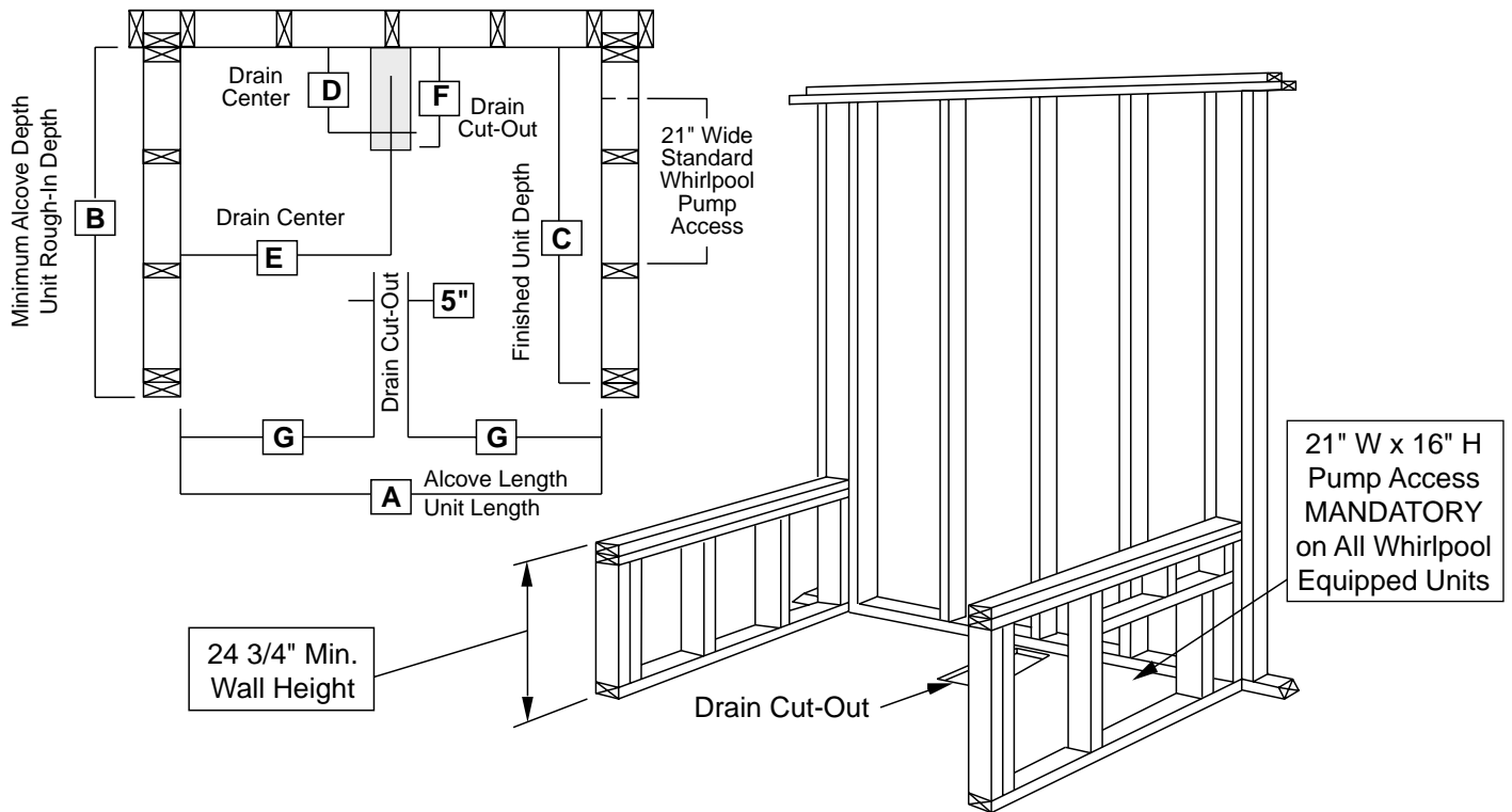
Figure 1 - Alcove Framing Guidelines
