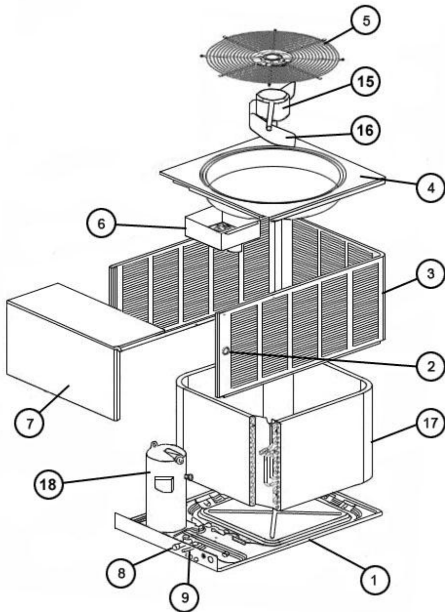
Exploded View
