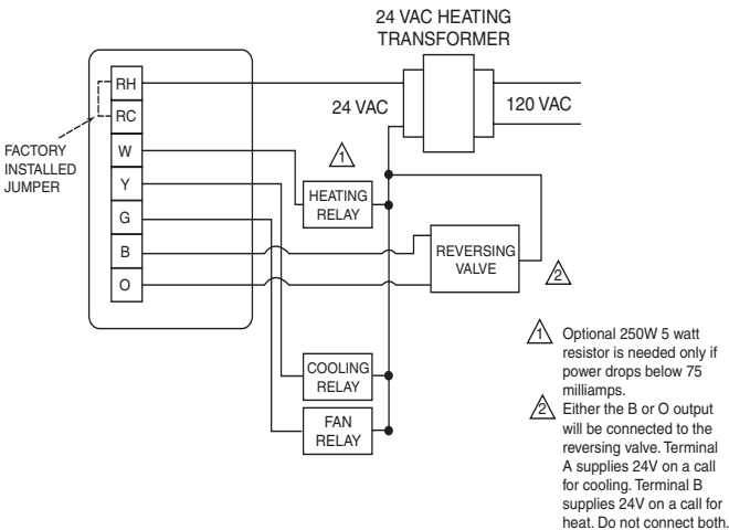
Figure 2 T207 Wiring to Heating/Cooling System With Single Transformer and Reversing Valve.
