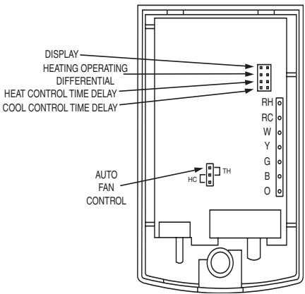
Figure 6 Terminal Identification.
