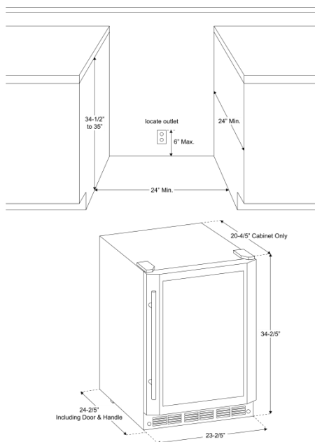
Figure A – The cutout depth must be 24"
