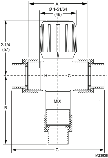
Fig. 4. Dimensions in in. (mm).
