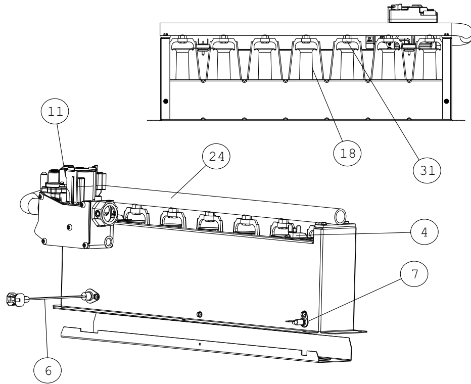
Figure 3: GAS CONTROLS
