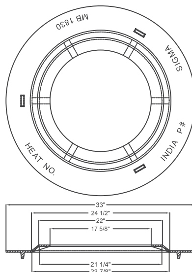
18" x 30" Adapter Ring Shipping Weight: 65 lbs.
