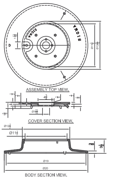
18" Frame and Cover w/ Touch Read Hole Shipping Weight: 29 lbs
