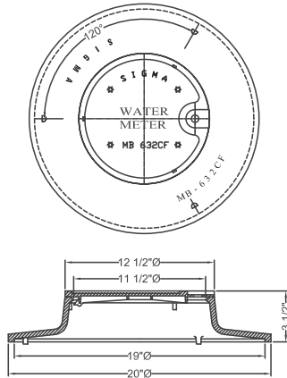
18" SIGMA Meter Box Frame and Cover Shipping Weight: 29 lbs
