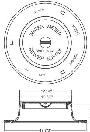
18" Meter Box Shipping Weight: 35 lbs
