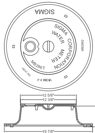
18" Meter Tile Ring and Cover with 2" AMR Shipping Weight: 35 lbs
