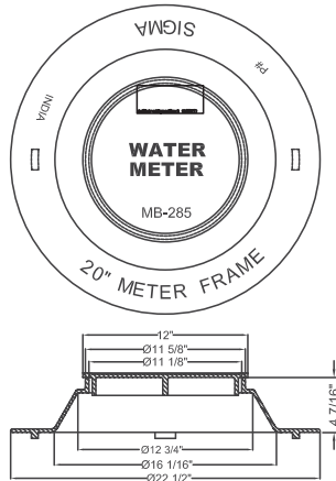
20" Meter Tile Ring and Cover Shipping Weight: 30 lbs
