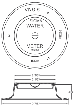
18" Meter Tile Ring and Cover Shipping Weight: 35 lbs
