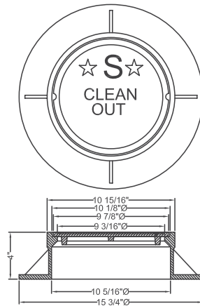
Clean Out Meter Box Shipping Weight: 31 lbs
