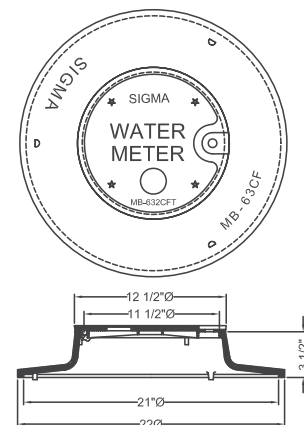
20" Meter Box Body and Cover with Touch Tone Hole Shipping Weight: 36.3 lbs
