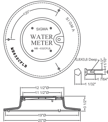
18" Body/Lid marked "Water Meter" with Pentagonal Long Bolt Shipping Weight: 29 lbs
