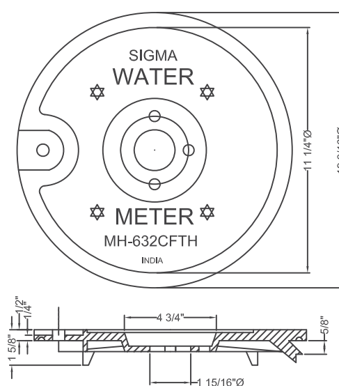
Cover for MB6732CFTH marked "Water Meter" w/ Touch Tone Hole Shipping Weight: 11.4 lbs
