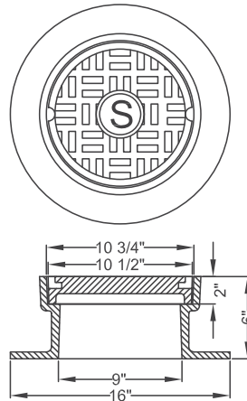
6" Lamphole Frame and Cover Shipping Weight: 50 lbs.
