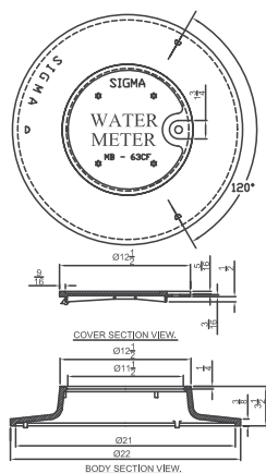
20" Meter Box Body and Cover Shipping Weight: 36.3 lbs
