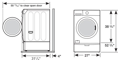
Required Dimensions for Installation With Pedestal
