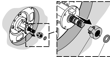
Collar/Collier/Collarín O-Ring/Joint torique/Arosello
