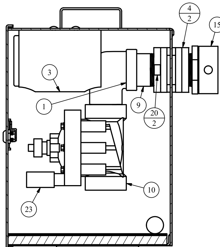
SECTION C-C SCALE 1 / 4
