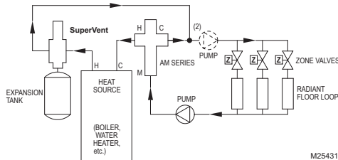
Fig. 5. Single Loop for Multiple Loops.
