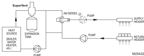
Fig. 6. AM-1 Primary/Secondary Application.
