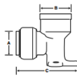
Drop Ear Elbow Dimensions
