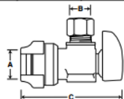
Angle Stop (Chrome Plated) Dimensions
