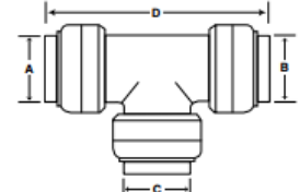
Tee Dimensions
