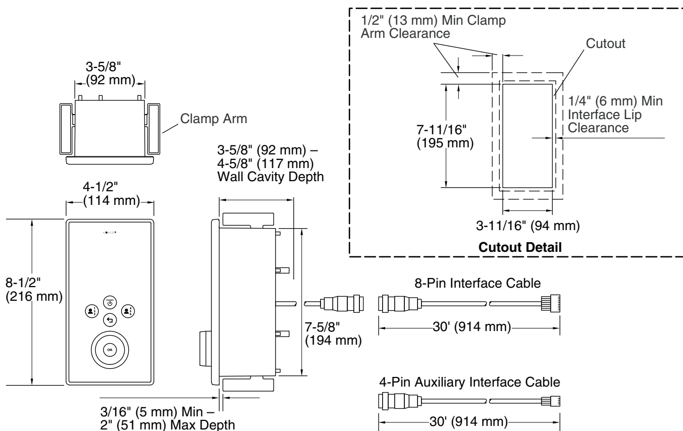
Product Diagram
