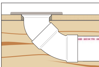
Using a standard 45° fitting, the Drop-Kick connects easily to horizontal drain lines.
