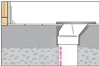
Correct Rough-in Mistake 1½" offset corrects for drain line set too close to wall.
