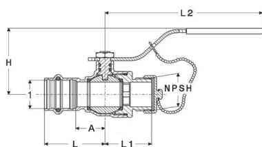
Viega ProPress Ball Valve Zero Lead Bronze P x Hose - Model 2971.5ZL
