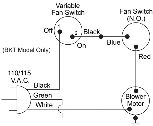
Figure 11 - Wiring Diagram
