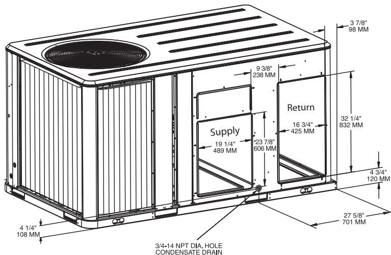
Figure 10. 4-5 ton High Efficiency R410a, 6-10 ton R22 and R410a Horizontal Unit Supply & Return Air Opening
