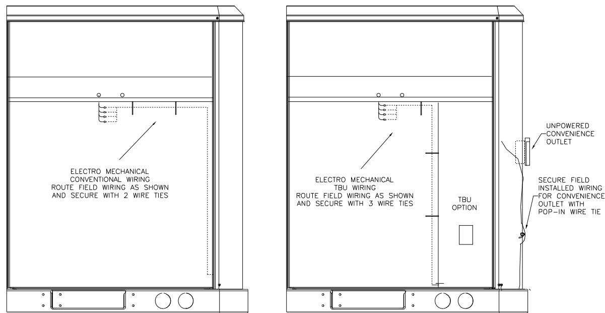
Figure 32. Electro mechanical control customer low voltage routing
