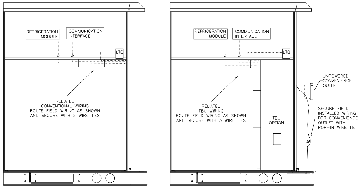
Figure 33. ReliaTel control customer low voltage routing
