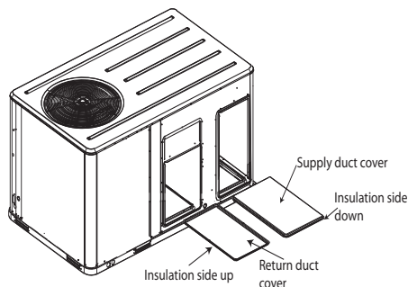
Figure 19. Duct cover
