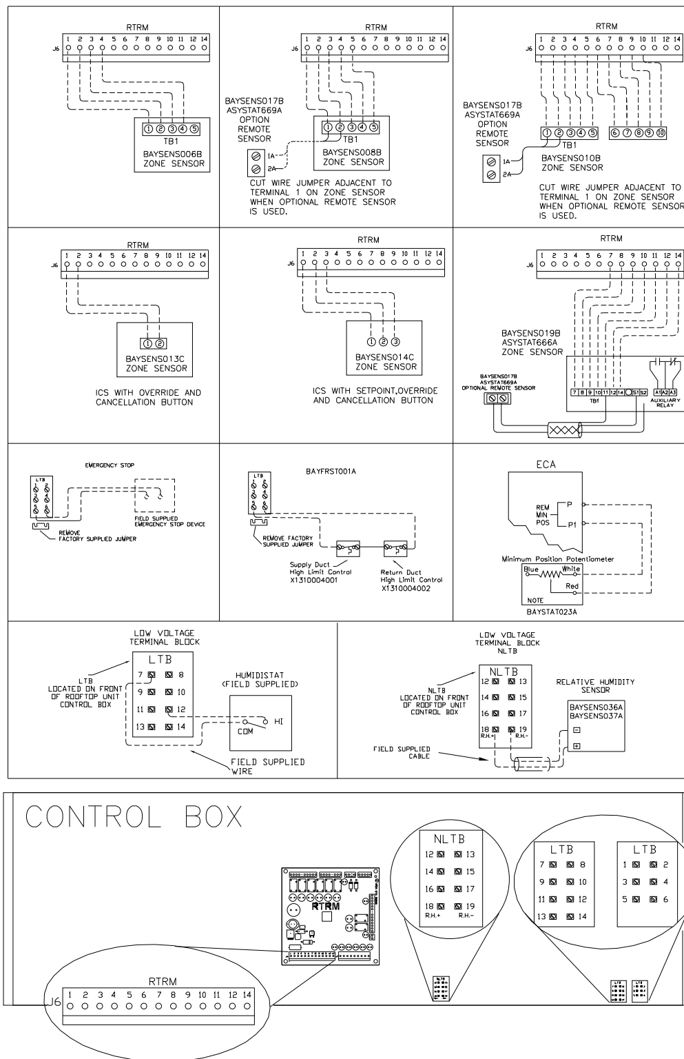
Figure 37. Typical field wiring diagrams for optional controls (ReliaTel only)
