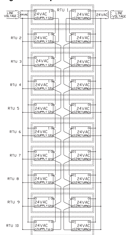
Figure 35. Up to 5 HVAC units
