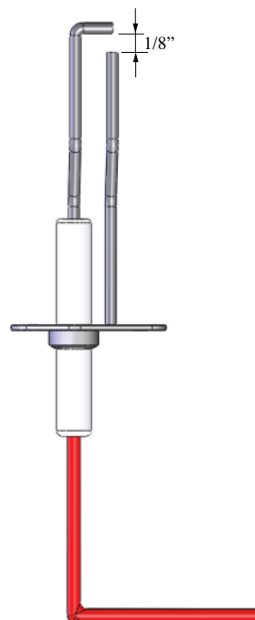
Fig. 3: Recommended Igniter Gap
