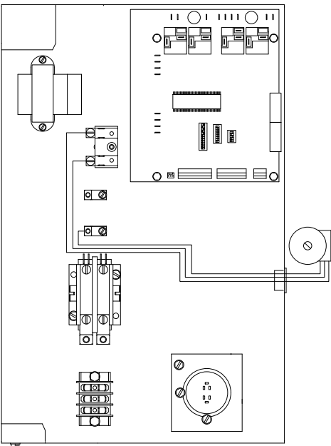
Figure 14: Pump Wiring 208-230/60/1
