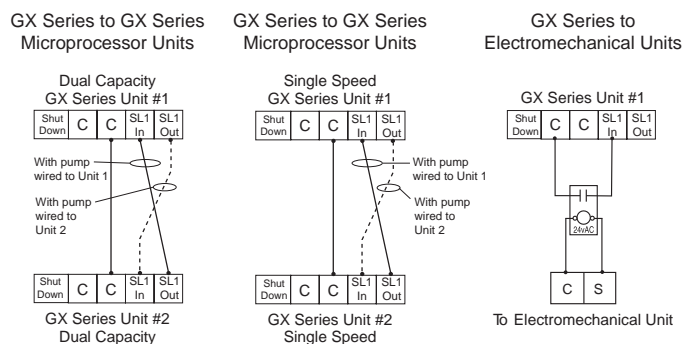
Figure 8: Primary/Secondary Hook-up
