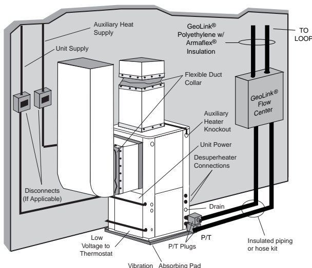
Figure 7: Closed Loop Ground Source Application
