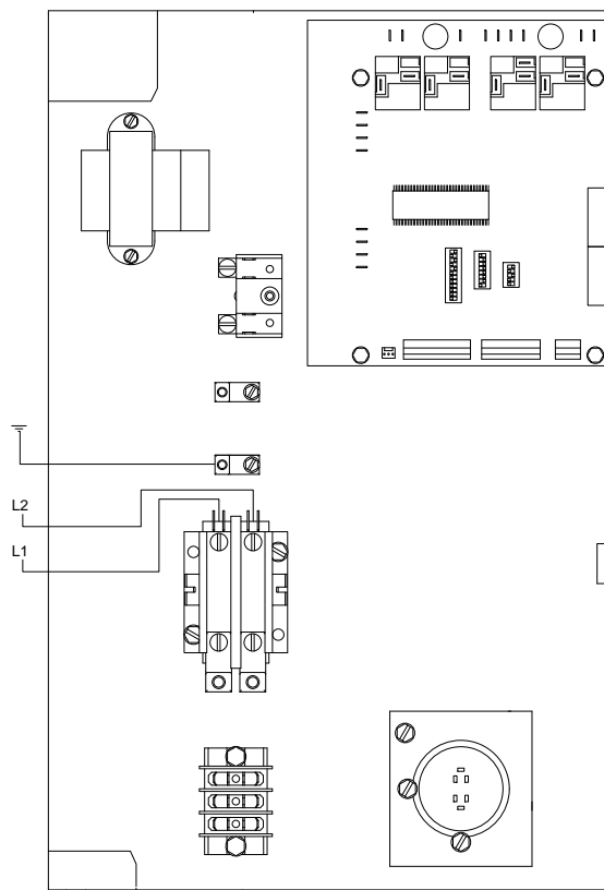
Figure 13B: Line Voltage 208-230/60/1 control box
