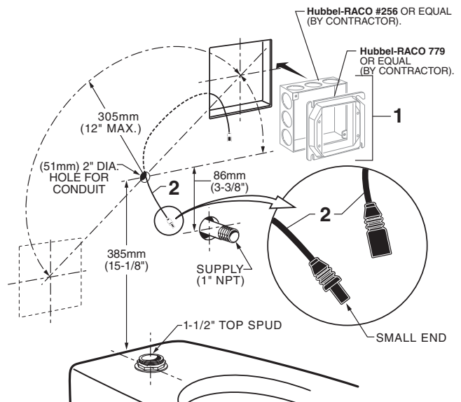
Fig.9 (TOP SPUD FIXTURE ILLUSTRATED)
