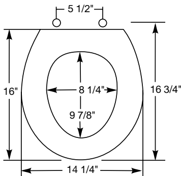
TOP-TITE® HINGES WITH BOLT AND WING NUT
