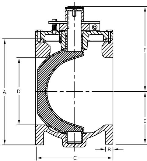
2-1/2" - 8" VALVES ONLY
