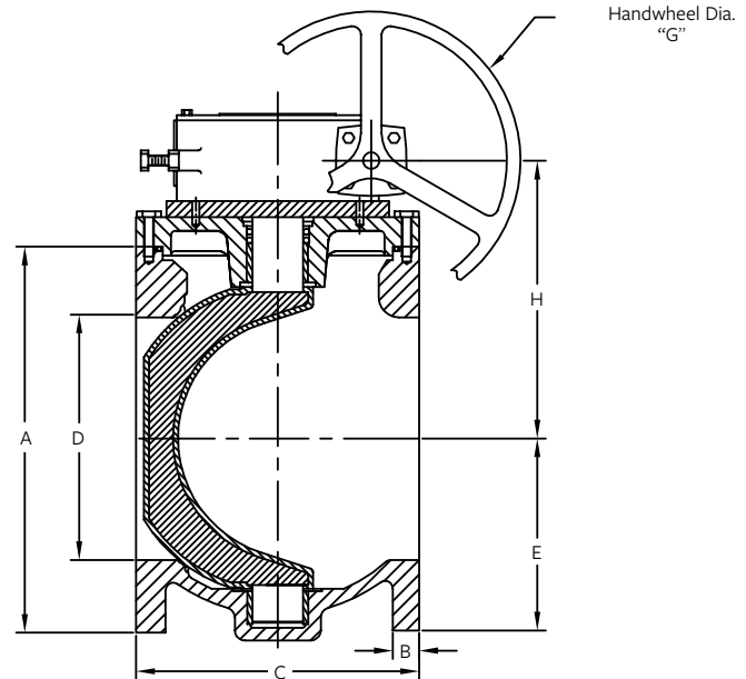
2-1/2" - 12" VALVES
