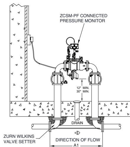
INDOOR INSTALLATION (475 with ZCSM-PF Connected Pressure Monitor Accessory)
