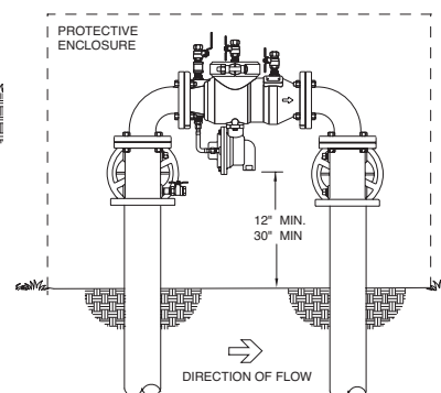
OUTDOOR INSTALLATION
